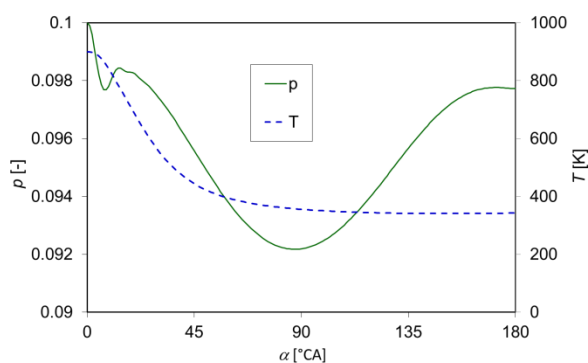
Fig. 7.2. Pressure and temperature in the gasoline engine cylinder during the intake process; V_s = 500 \text{ cm}^3 , n = 6000 \text{ 1/min} , full load
