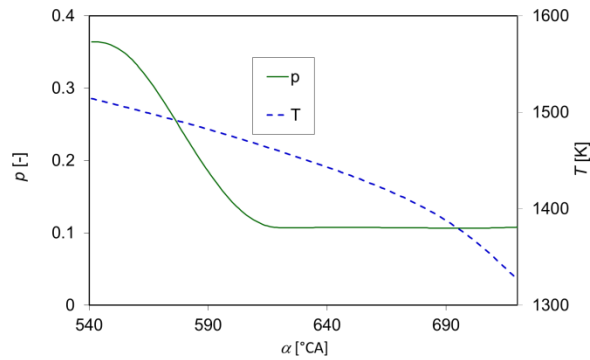
Fig. 9.3. In-cylinder pressure and temperature in the gasoline engine during the exhaust process; V_s = 500 \text{ cm}^3 , n = 6000 \text{ 1/min} , full load
