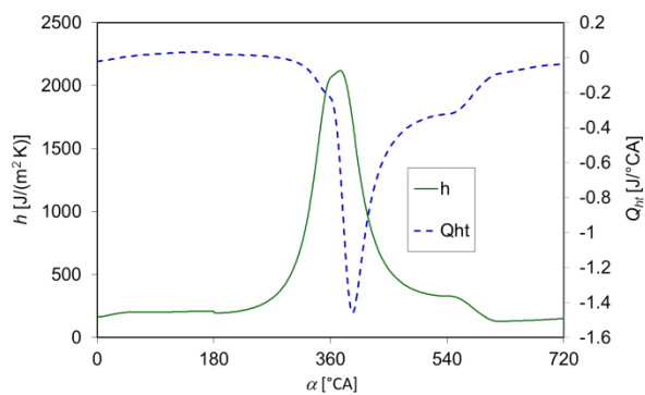
Fig. 10.1. Heat transfer coefficient and heat flow during full work cycle of the gasoline engine; V_s = 500 \text{ cm}^3 , n = 6000 \text{ 1/min} , full load, T_w = 500 \text{ K}
