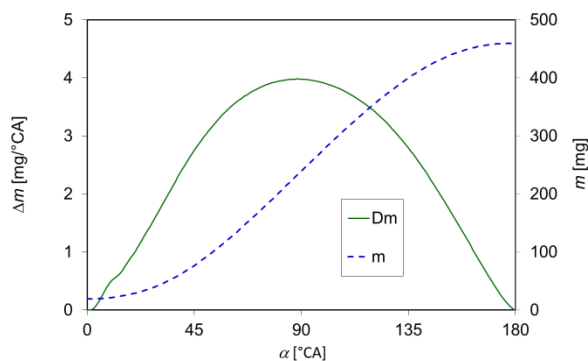
Fig. 7.2. Mass flow rate and cumulated mass in the gasoline engine cylinder during the intake process; V_s = 500 \text{ cm}^3 , n = 6000 \text{ 1/min} , full load
